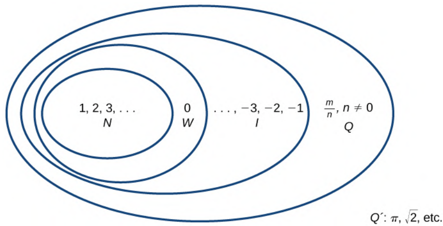
Figure 2 Sets of numbers
