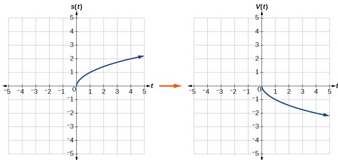
Figure 13 Vertical reflection of the square root function
