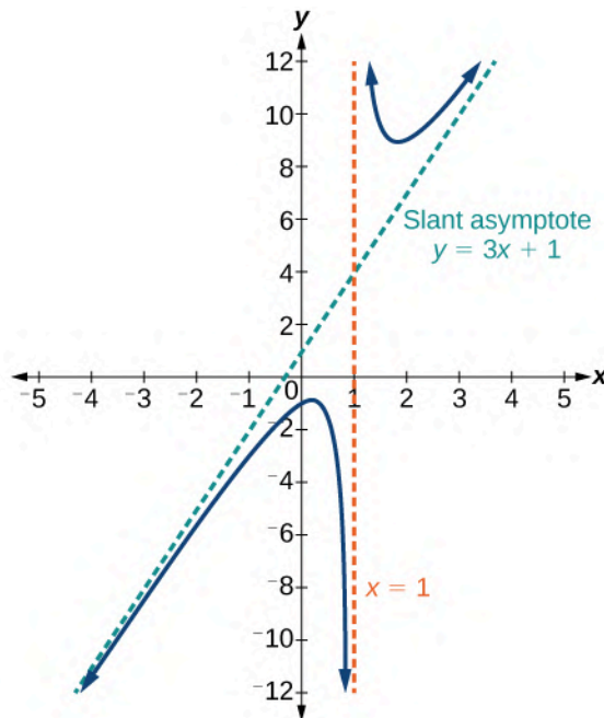
Figure 13 Slant asymptote when f(x) = \frac{p(x)}{q(x)} , q(x) \neq 0 where degree of p > degree of q by 1.
