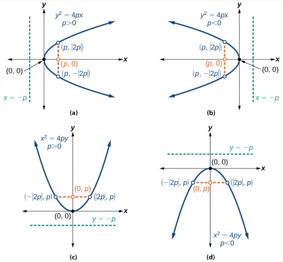
Figure 5 (a) When p > 0 and the axis of symmetry is the x-axis, the parabola opens right. (b) When p < 0 and the axis of symmetry is the x-axis, the parabola opens left. (c) When p > 0 and the axis of symmetry is the y-axis, the parabola opens up. (d) When p < 0 and the axis of symmetry is the y-axis, the parabola opens down.
