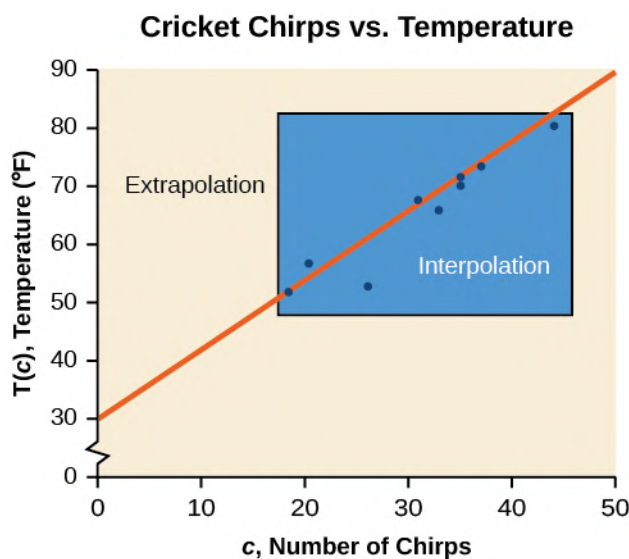
Figure 4 Interpolation occurs within the domain and range of the provided data whereas extrapolation occurs outside.
